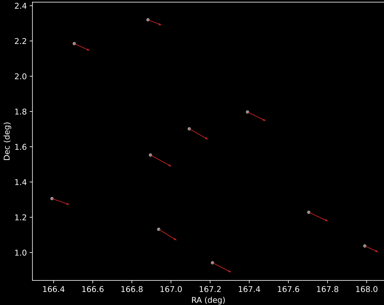
GALAH DR4 Cluster 6 Proper Motion Vectors (n=10)
