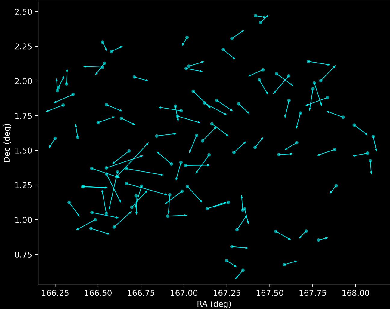
GALAH DR4 Noise Stream Proper Motion Vectors (n=94)
