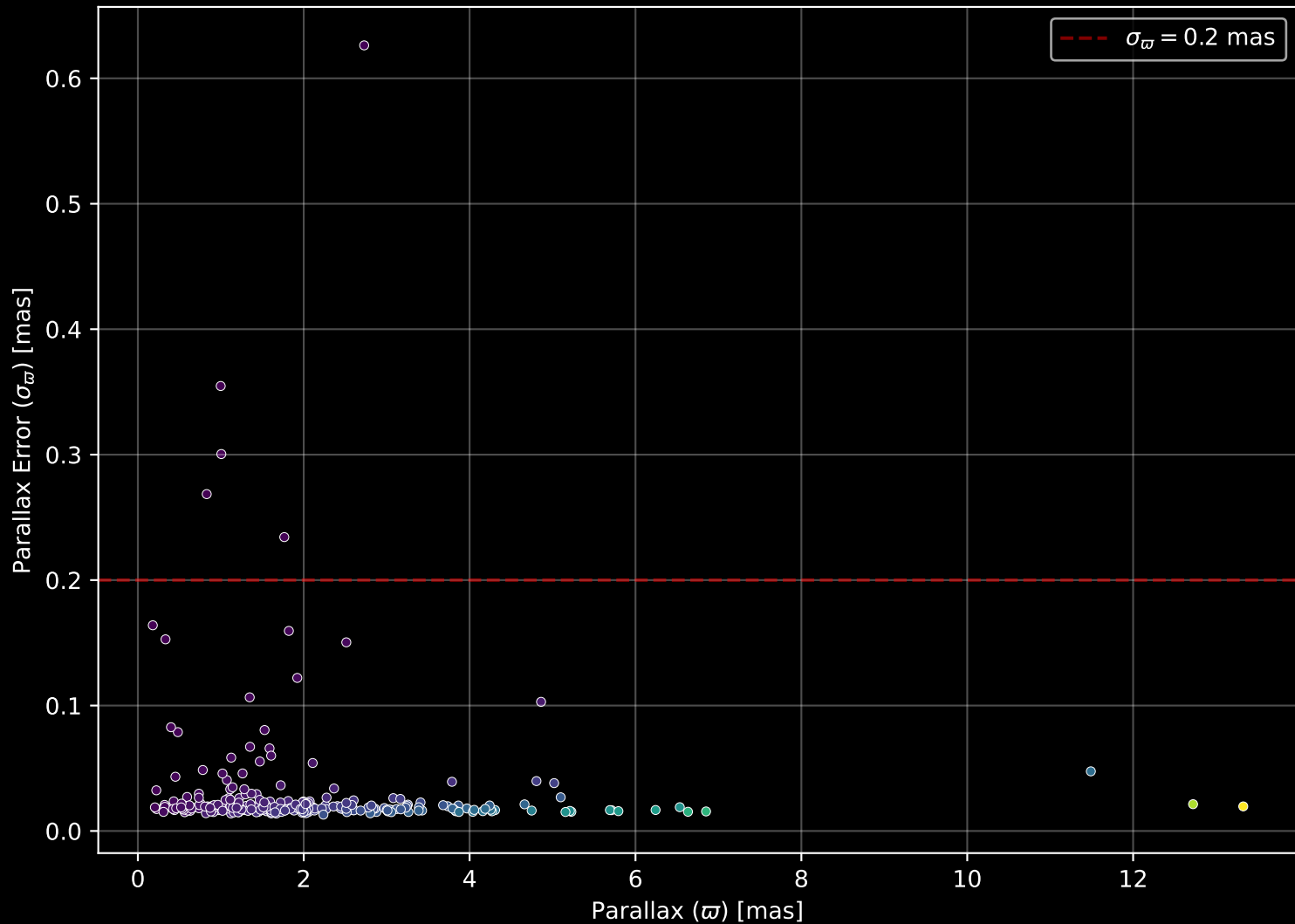
GALAH DR4 Field: [945] Parallax Quality (n= 284)
