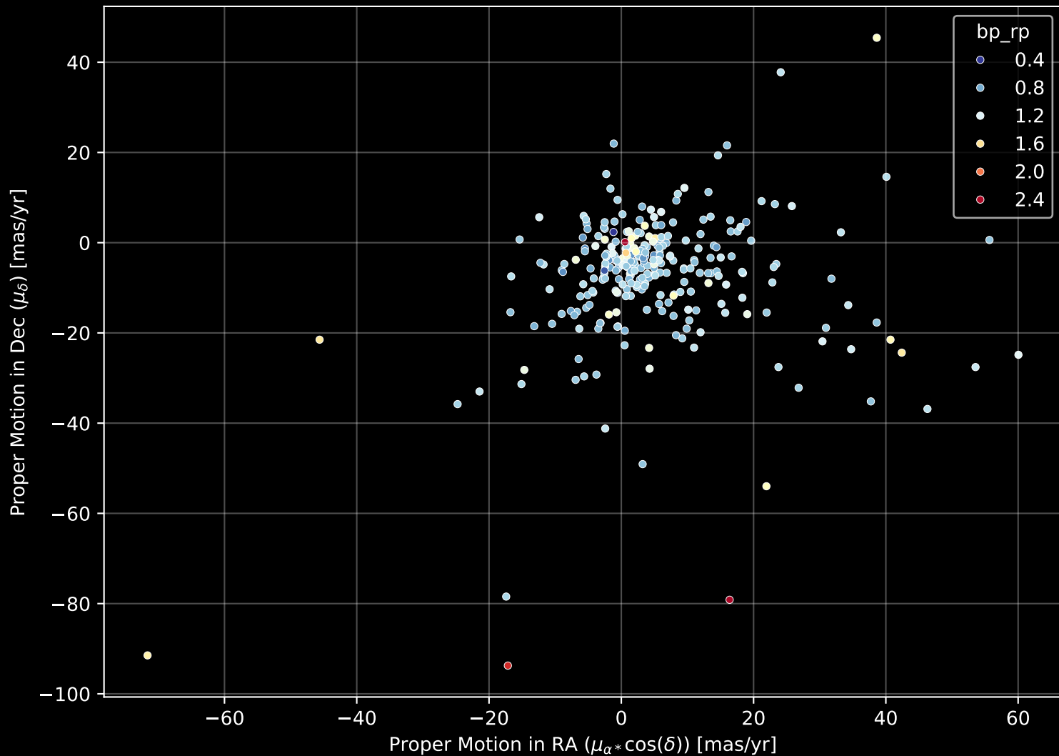
GALAH DR4 Field: [945] Proper Motion Diagram (n= 284)
