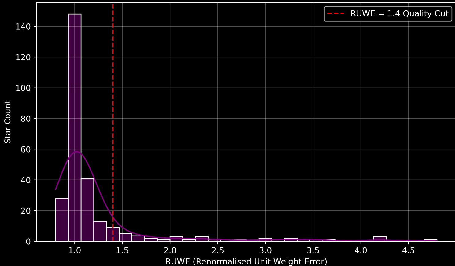
GALAH DR4 Field [945] RUWE Distribution (n= 271)
