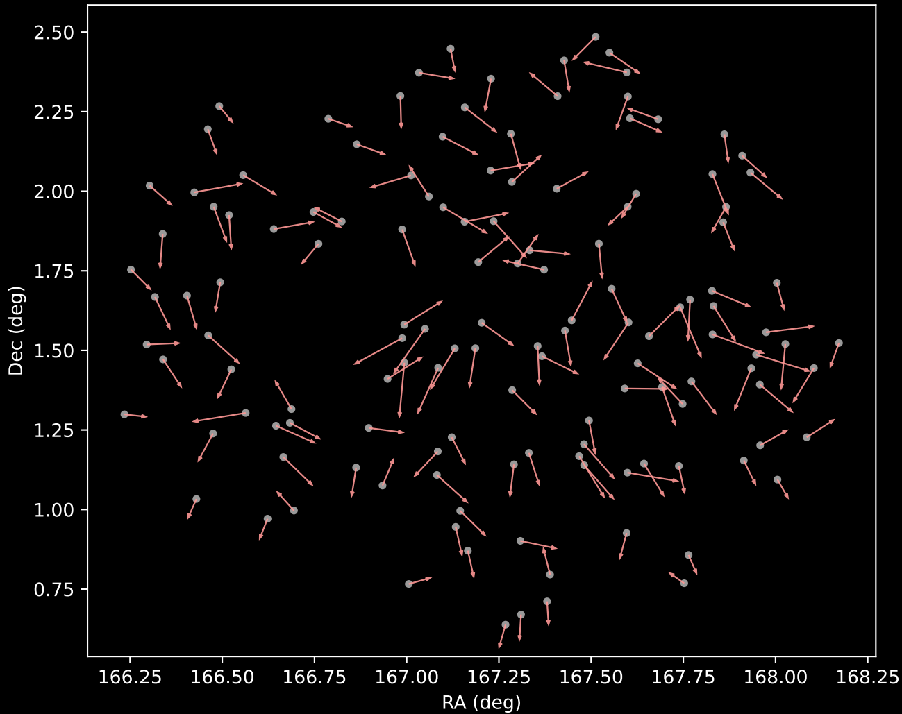
GALAH DR4 Cluster 7 Proper Motion Vectors (n=135)
