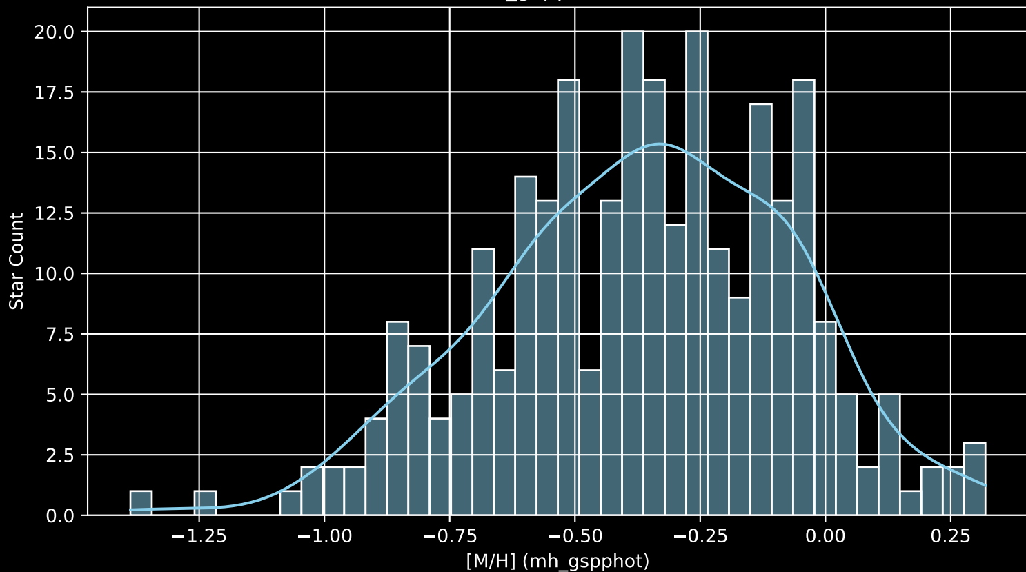
GALAH DR4 Field: [945] [M/H] (mh_gspphot) (n= 284)
