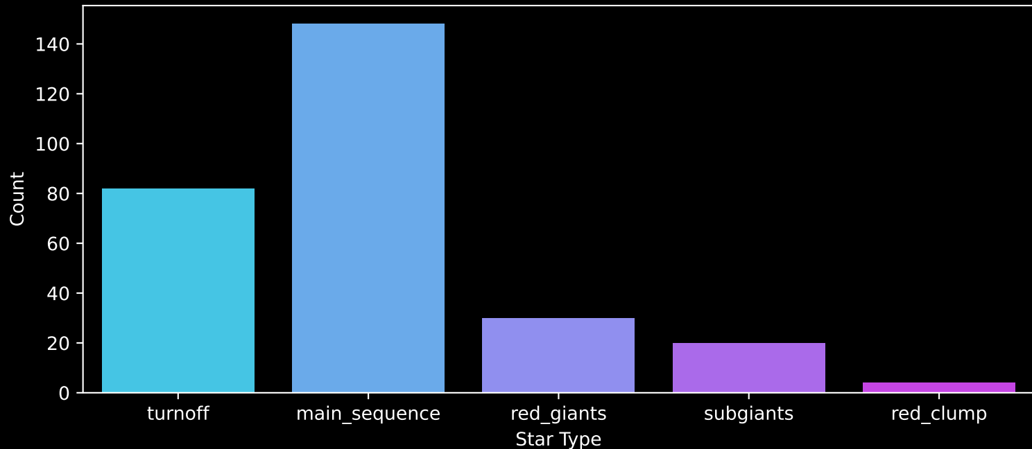
GALAH DR4 Field: [945] Count plot of Star Type
