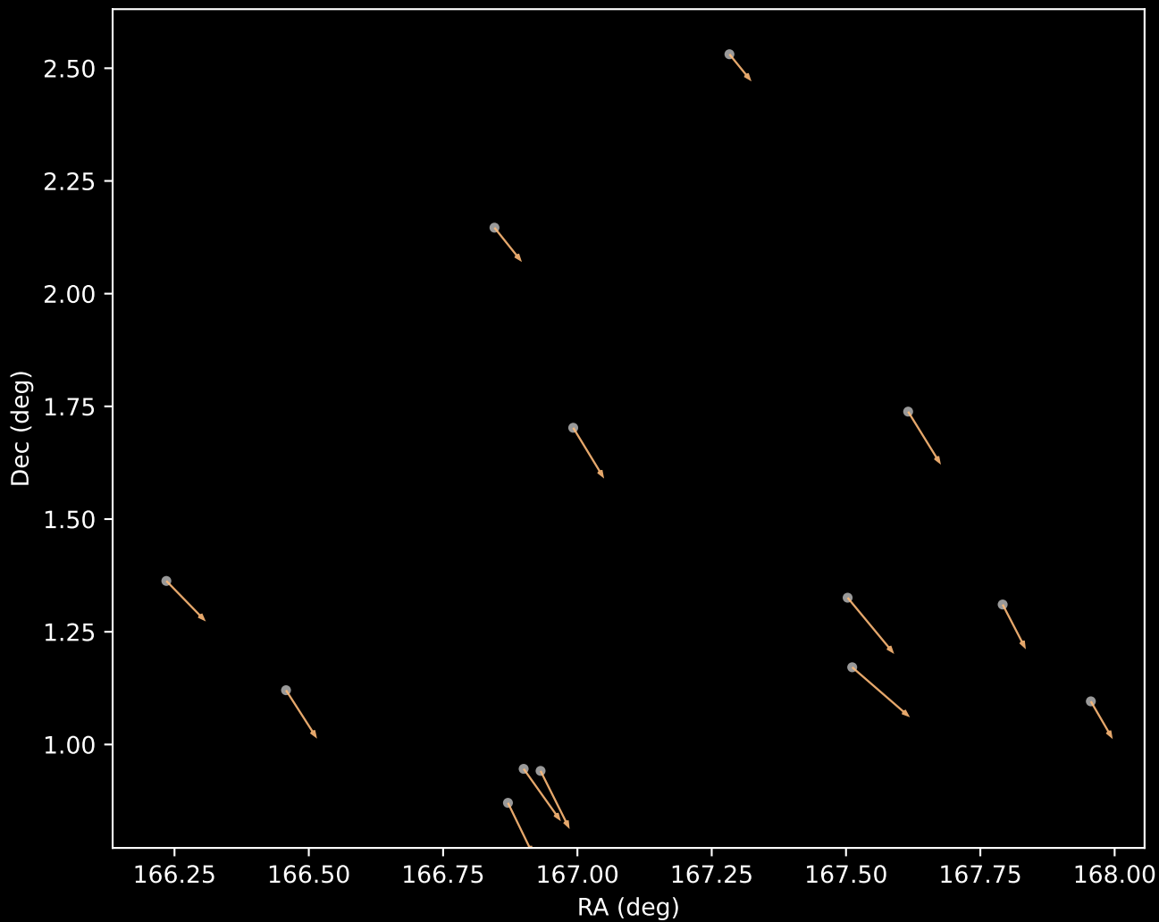
GALAH DR4 Cluster 3 Proper Motion Vectors (n=13)
